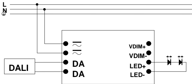
DALI Control
